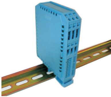
Type ZBPD din rail mounting Zener Barrier with external dimensions of 102 x 76 x 23mm.
